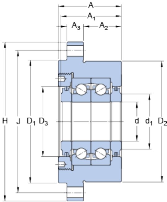
FBSA 208/DF Bearing 2D drawings and 3D CAD models
